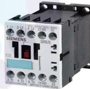
4 Pole Power Contactors
